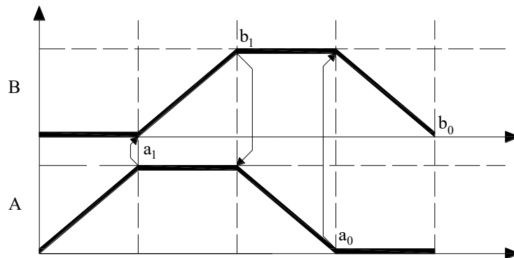
Figure 3. Generation of a suitable “Movement-Phase” displacement
